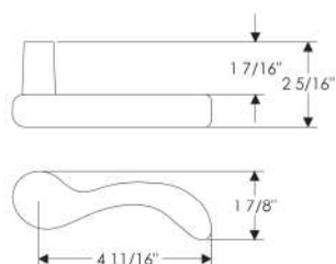
L119 Long Legacy Lever
