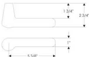
L163 Euro Lever
