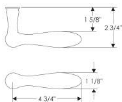
L158 Large Acanthus Lever
