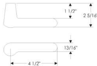
L127 Scroll Lever
