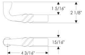
L132 Square Twist Lever
