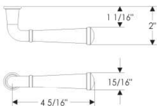
L160 Wing Lever
