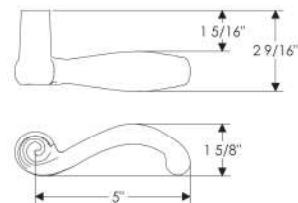
L132 Square Twist Lever
