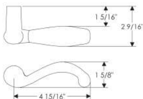
L117 French Lever
